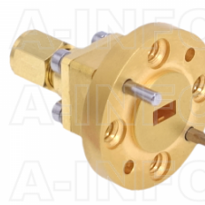
15WECA1.0M_Cu Endlaunch Rectangular Waveguide to Coaxial Adapter 50-75GHz WR15 to 1.0mm Male
