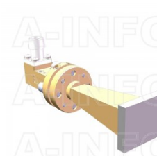
LB-15-15-C-1.85FSPO Standard Gain Horn Antenna 50-65GHz 15dB Gain 1.85mm Female
